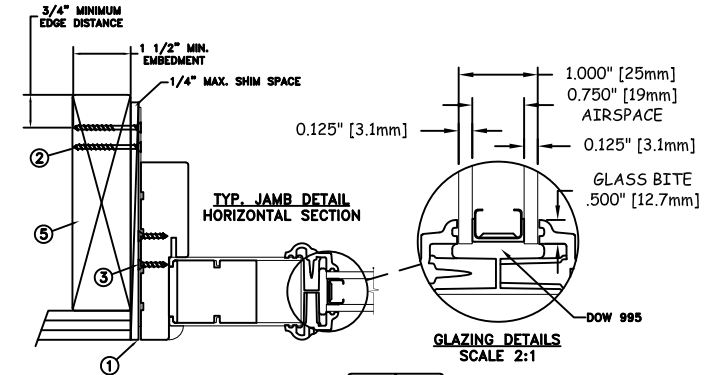
TYP. MULLION DETAIL HORIZONTAL SECTION
