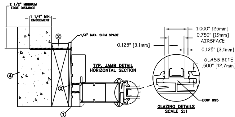
TYP. MULLION DETAIL HORIZONTAL SECTION
